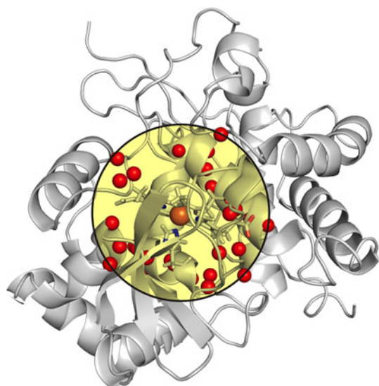
Fig. 1 The “blind spot” in the NMR resonance assignments of the high-spin CcP. The highlighted region shows HN atoms (red spheres) located within 11 Å from the heme iron (orange sphere). These protons are not observed in the NMR spectra of the CcP-RS due to large PREs caused by the high-spin ( S = 5/2 ) Fe(III) atom. The heme group is shown in sticks
