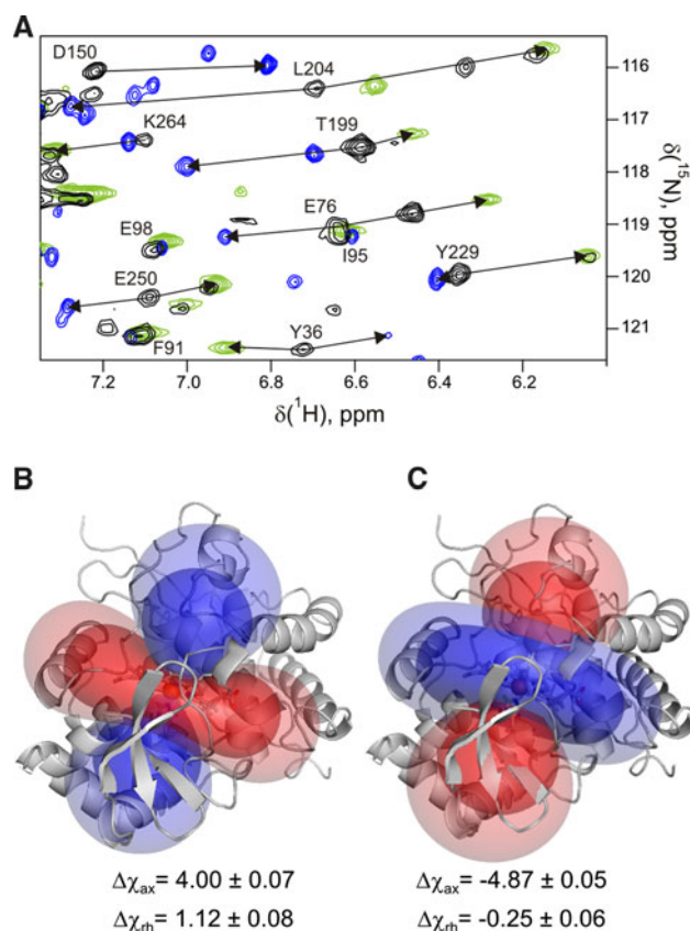
Fig. 2 Paramagnetic properties of the CcP in different spin-states. a A region of the overlaid [^1\text{H}, ^{15}\text{N}] TROSY spectra of the CcP-PPIX (black), CcP-CN (blue), and CcP-RS (green), with the arrows indicating PCSs of several backbone amides identified by the labels. Experimentally determined \Delta\chi tensors of the b low-spin CcP-CN and c high-spin CcP-RS. The \Delta\chi are in 10^{-32} \text{ m}^3 . The blue and red isosurfaces indicate positive and negative PCSs of \pm 0.5 ppm (dark shade) and \pm 0.2 ppm (light shade), respectively. The protein is in the same orientation as in Fig. 1
